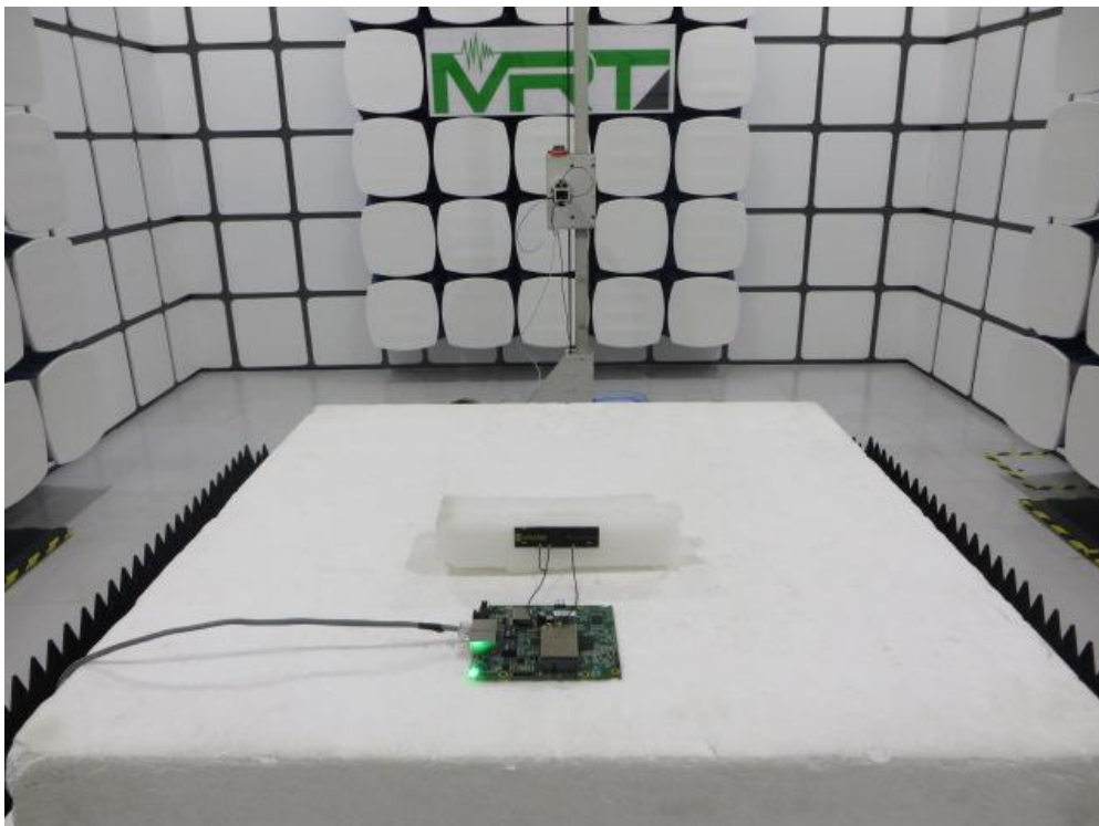
Description: Radiated Spurious Emissions Test Setup for 18 - 40GHz
